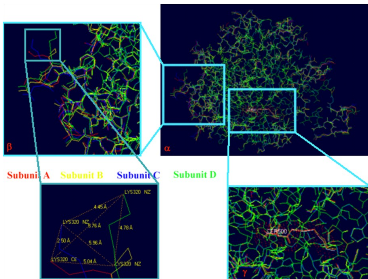
Figure 6. Different views of the superimposition of the four subunits of the KAS I enzyme with cerulenin docked (pdb entry: 1FJ8).
