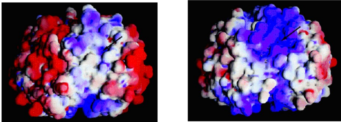
Figure 7. Accessible surface map representation of electrostatic potential distribution on the KAS I and KAS II dimer, respectively. Positive and negative electrostatic potentials are colored blue and red, respectively. Notice that the overall distribution of charges is the same: Positive potential around the active site flanked by strong negative potential. An arrow points to the active site entrances.
